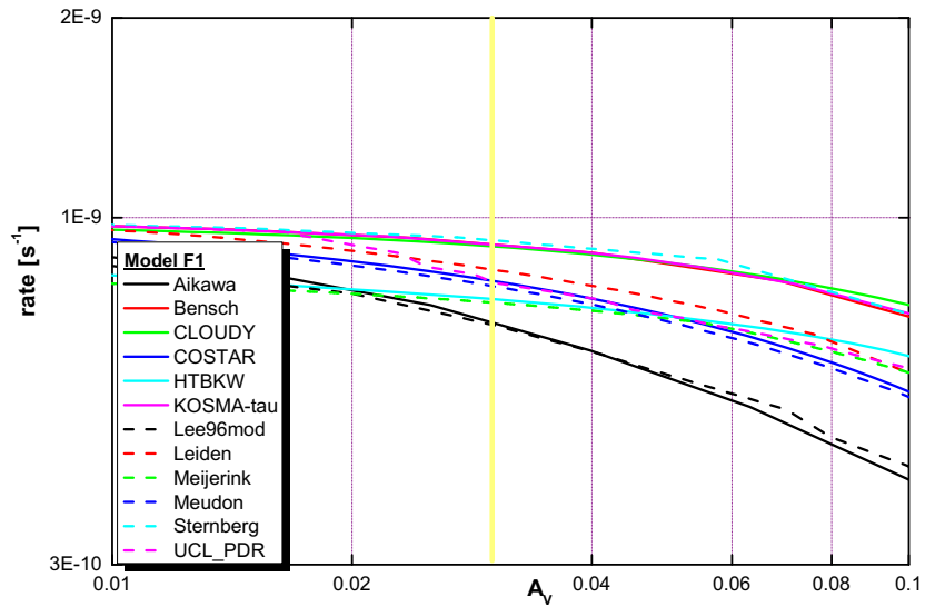
CO photodissociation rate - n = 10^3 \text{ cm}^{-3} , \chi = 10
