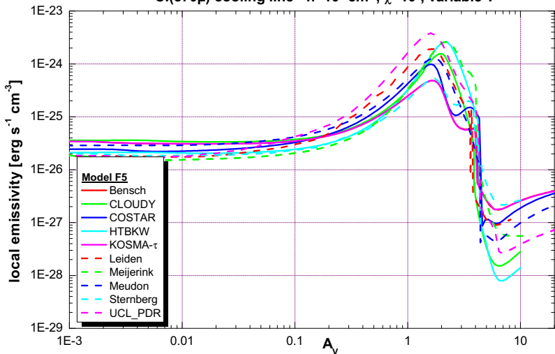
Cl(370 \mu ) cooling line - n=10^3 \text{ cm}^{-3} , \chi=10^1 , variable T
