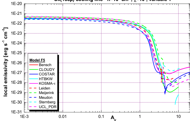
ClI(158 \mu ) cooling line - n=10^3 \text{ cm}^{-3} , \chi=10^1 , variable T
