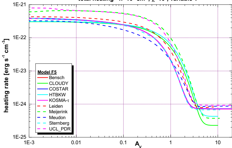
total heating - n=10^3 \text{ cm}^{-3} , \chi=10^1 , variable T
