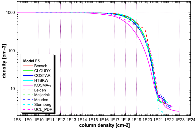
n(\text{H}) vs. N(\text{H}_2) - n=10^3 \text{ cm}^{-3} , \chi=10^1 , variable T
