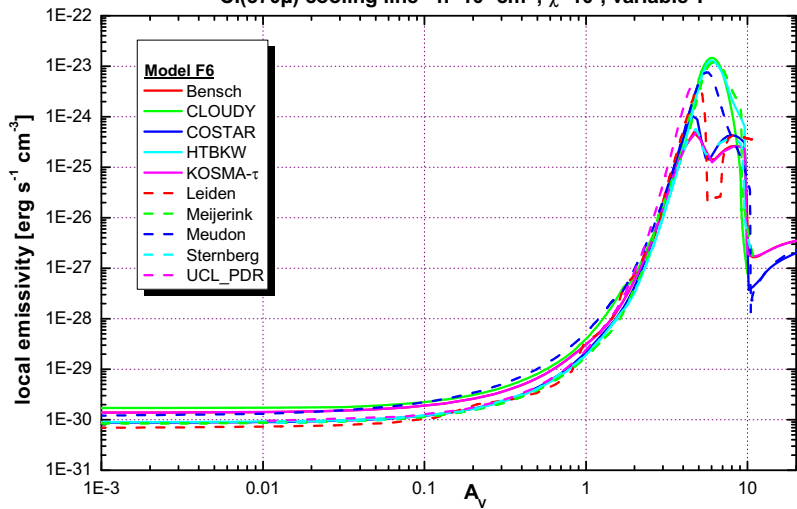
CI(370 \mu ) cooling line - n=10^3 cm ^{-3} , \chi=10^5 , variable T
