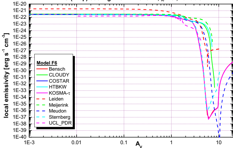
OI(146 \mu ) cooling line - n=10^3 \text{ cm}^{-3} , \chi=10^5 , variable T
