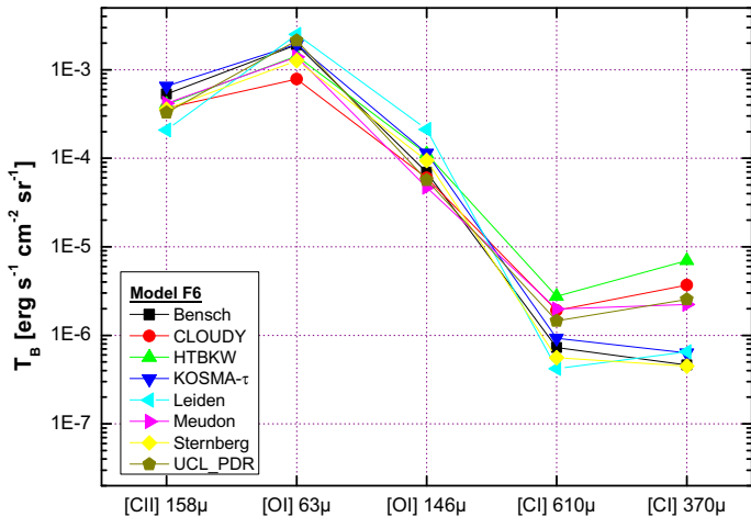
surface brightness - n=10^3 \text{ cm}^{-3} , \chi = 10^5 , variable T
