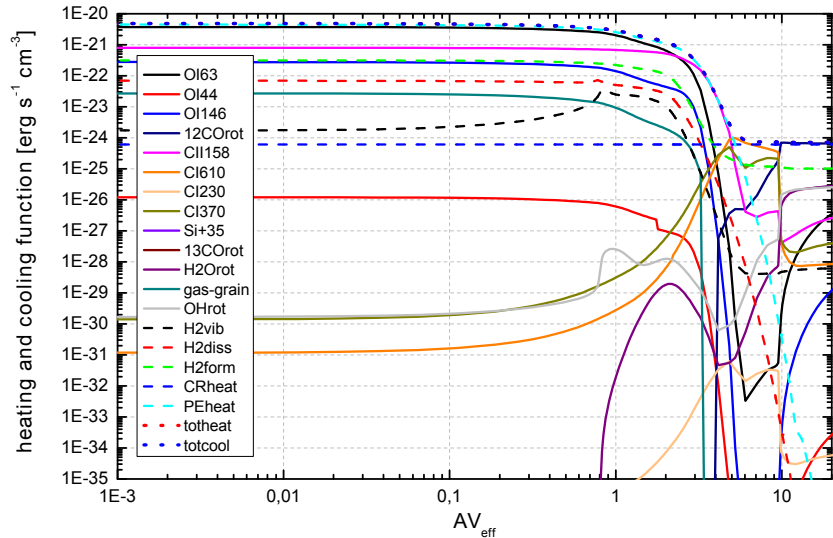
KOSMA-tau Model F6 - all cooling and heating functions
