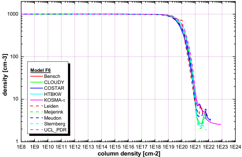
n(\text{H}) vs. N(\text{H}_2) - n=10^3 \text{ cm}^{-3} , \chi=10^5 , variable T
