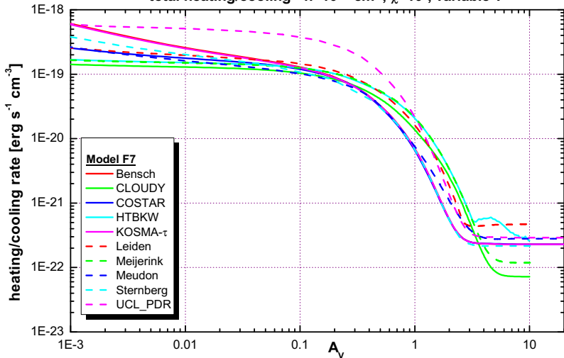
total heating/cooling - n=10^{5.5} \text{ cm}^{-3} , \chi=10^1 , variable T
